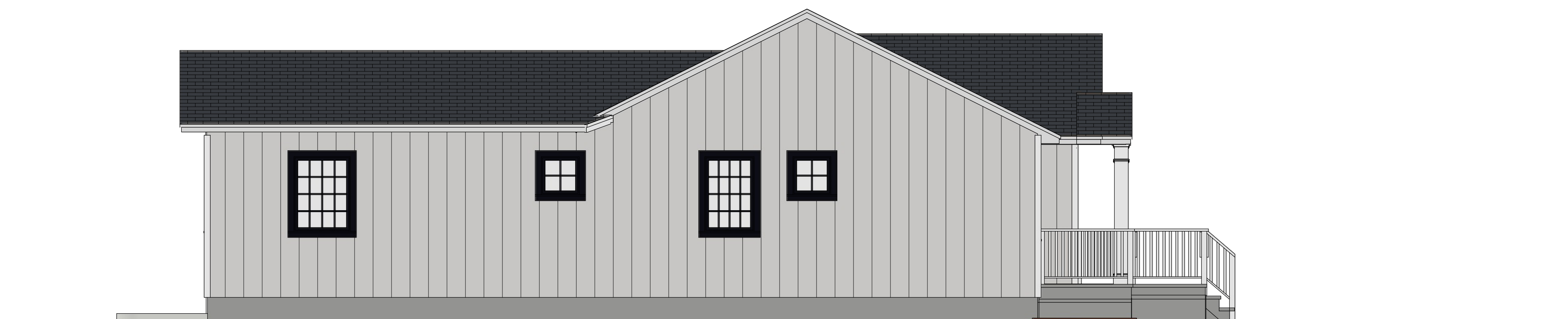
LEFT DESIGN ELEVATION SCALE: 1/4" = 1'-0"
