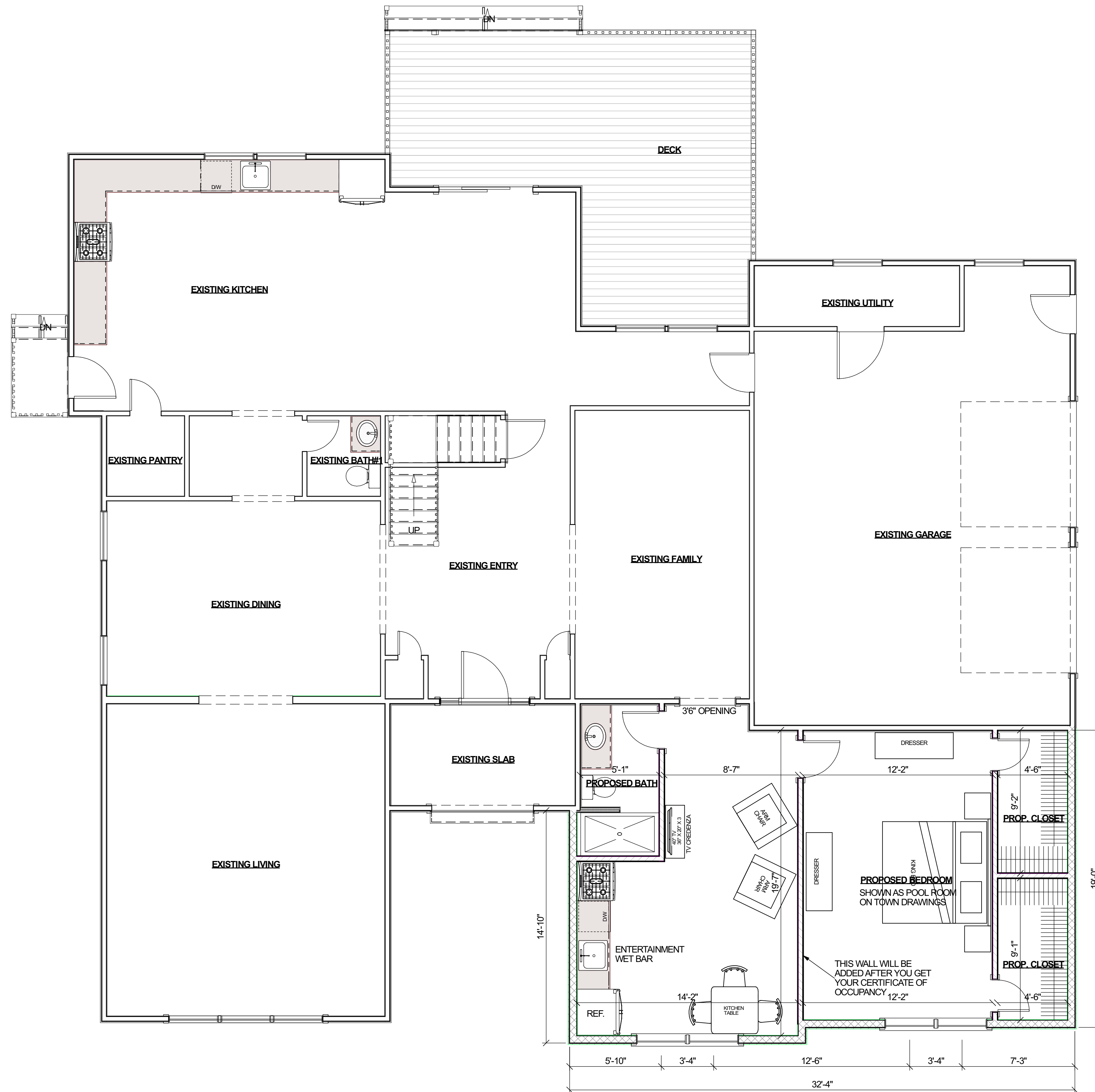
FIRST FLOOR DESIGN PLAN SCALE: 1/4" = 1'-0"
