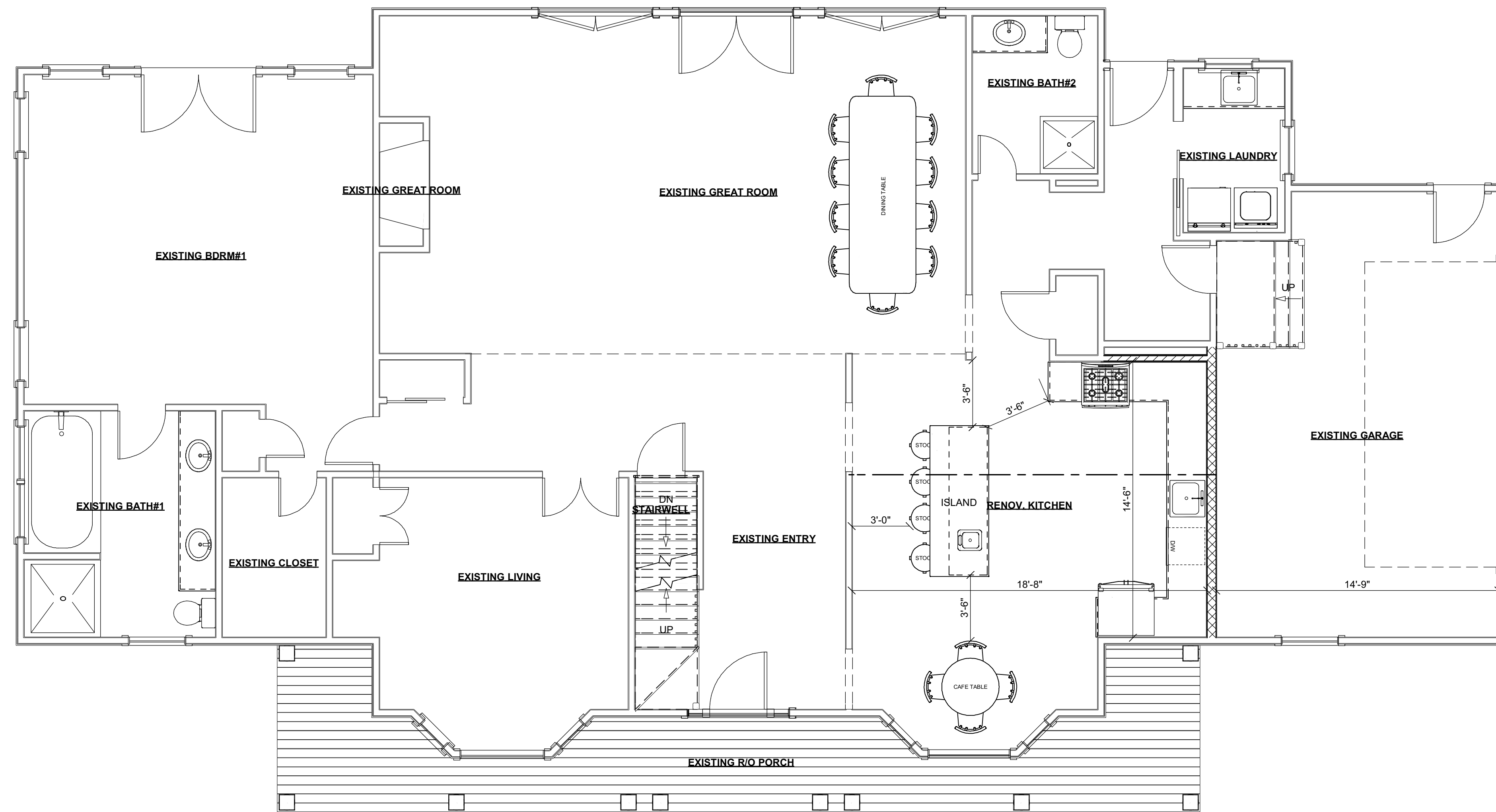
MEYERS DESIGN 2 FIRST FLOOR DESIGN PLAN SCALE: 1/4" = 1'-0"
